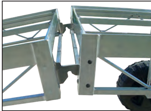
Dual-Stage Hook System
