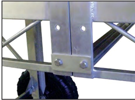
Standard Bolt System
